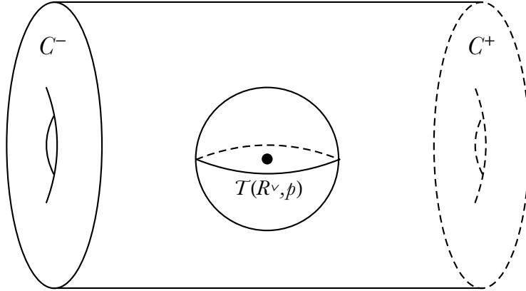
Figure 6.2: An illustration of how the insertion of a ‘t Hooft operator of type \check{R} equivalently gives rise to a cobordism C^- \sqcup \mathbb{C}\mathbb{P}^1 \rightarrow C^+ with boundary conditions on S^2 arising from the G -bundle on \mathbb{C}\mathbb{P}^1 induced by \check{R} .
